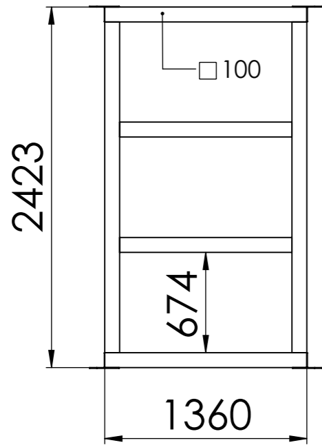
INSTALLATION FRAME
