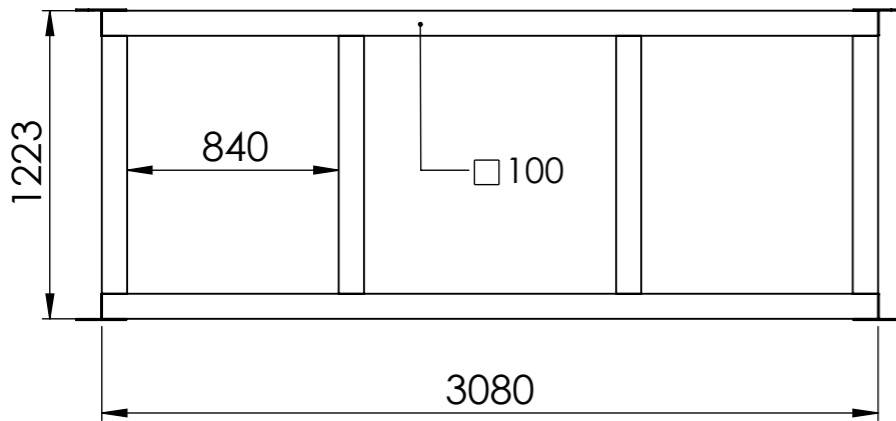
INSTALLATION FRAME
