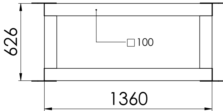
INSTALLATION FRAME
